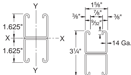
ELEMENTS OF SECTION - PS 210 2T3
