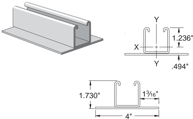
ELEMENTS OF SECTION
