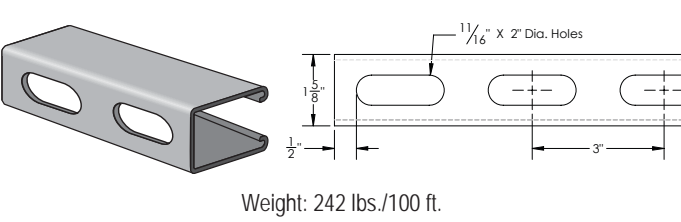
ELEMENTS OF SECTION – PS 150 2T3
