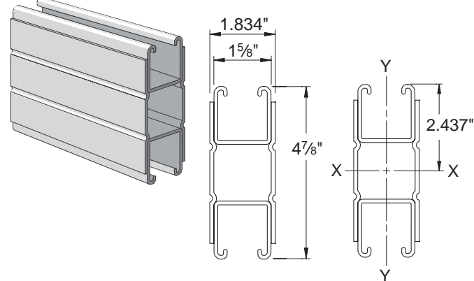
ELEMENTS OF SECTION
