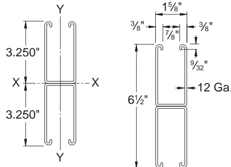
ELEMENTS OF SECTION - PS 100 2T3
