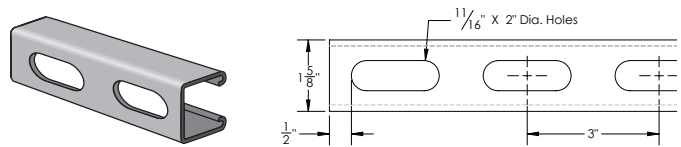
ELEMENTS OF SECTION - PS 200 2T3
